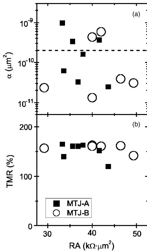
FIG. 3. Normalized noise measured at +200 mV (a) and zero-bias TMR (b) as a function of RA product. The dashed line (part a) indicates the lowest Hooqe factor value previously reported for MTJs with RA product within the wide range between 10^{-4} and 10^3 \text{ M}\Omega \mu\text{m}^2 (see Ref. 13).
